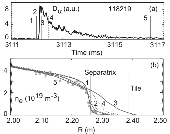
Fig. 1. Profile evolution during a single ELM, showing: (a) divertor D_z signal, where the numbers and vertical lines represent the times for the density profile sequence shown in (b). The points with error bars in (b) are Thomson scattering data taken at the same time as profile 5.
